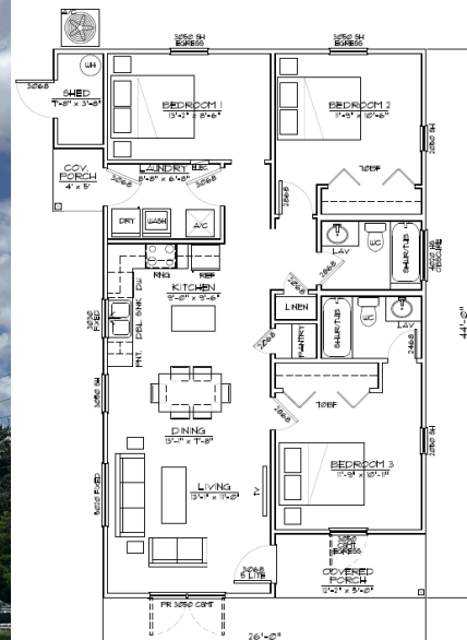
FLOOR PLAN 10'0" x 12'0" 10'0" x 12'0" 10'0" x 12'0" 12'0" x 12'0" 10'0" x 10'0" 10'0" x 10'0" 5'0" x 7'0" 5'0" x 7'0" 10'0" x 10'0" 4'0" x 6'0"
