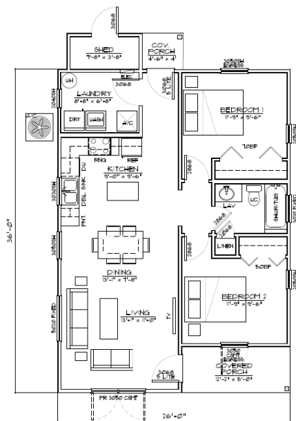
FLOOR PLAN 14' x 7'-6" LIVING 874 SQ. FT. SHED 34 SQ. FT. PORCHES 60 SQ. FT.
