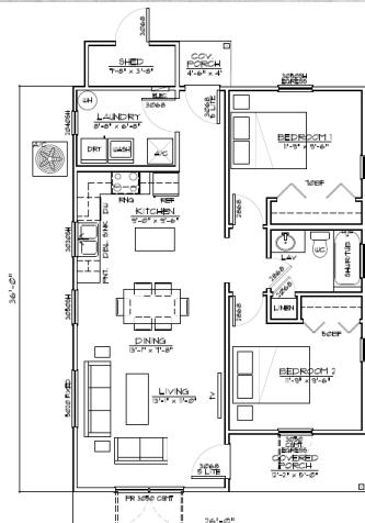
FLOOR PLAN 14'0" x 27'0" LIVING 874 SQ. FT. 14'0" x 27'0" BATH 14 SQ. FT. 14'0" x 27'0" PORCH 65 SQ. FT.
